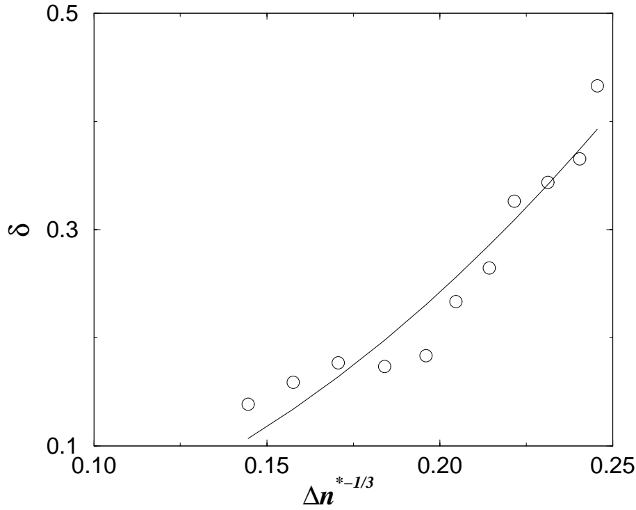
FIGURE 5.13 The difference \delta = R_e - R_s between the equimolar dividing surface and the surface of tension as function of the excess number of particles, \Delta n^{*-1/3} , in the critical nuclei. The solid curve is a fit of the data to a function of the form f(\Delta n^{*-1/3}) = c_1 \Delta n^{*-1/3} + c_2 \Delta n^{*-2/3} . This corresponds to a Tolman length \delta_T = \lim_{\Delta n^{*-1/3} \rightarrow 0} \delta = 0.0 , as (implicitly) assumed in the non-uniform droplet model of McGraw and Laaksonen [13]. Clearly, our simulations do not rule out this possibility.
