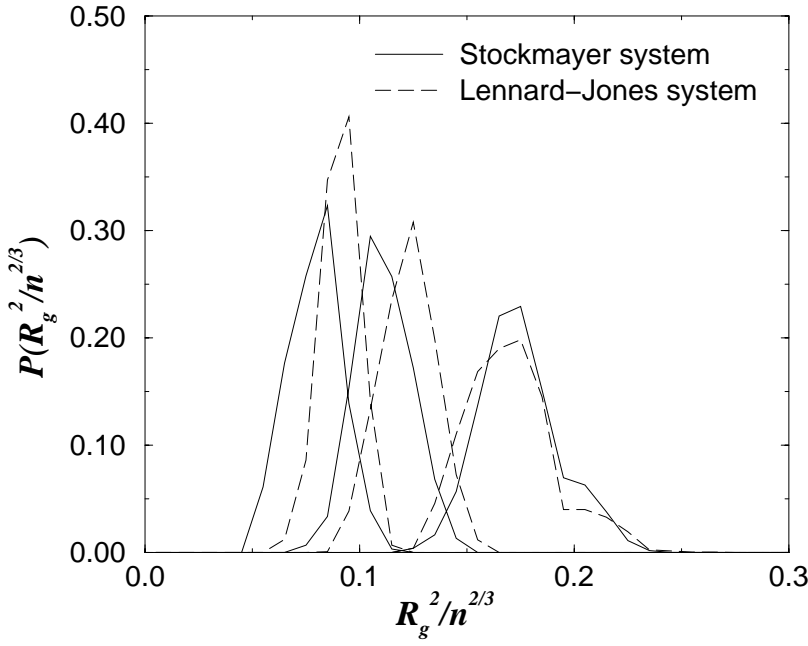
FIGURE 8.5 The distribution functions of the three eigenvalues of the moment-of-inertia tensor for a cluster of around 300 particles in a Stockmayer system at T^* = 3.5 ( = 0.7T_c ) and S = 1.26 . For comparison we also show the distribution functions for a Lennard-Jones cluster of comparable size ( n \approx 300 ) and at the same temperature with respect to the critical temperature ( T = 0.7T_c ). In this and subsequent figures \sigma is the unit of length.
