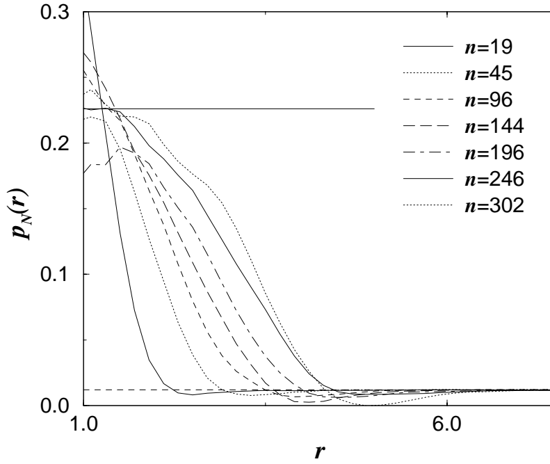
FIGURE 5.4 Radial profiles of the normal component of the pressure tensor, p_N(r) , for several precritical and critical nuclei at a supersaturation of S = 1.53 ( T = 0.741 , P = 0.01202 ). The thin horizontal dashed line denotes the pressure in the bulk vapor and the thin horizontal solid line denotes the pressure in the bulk liquid, which has a chemical potential equal to that of the vapor phase.
