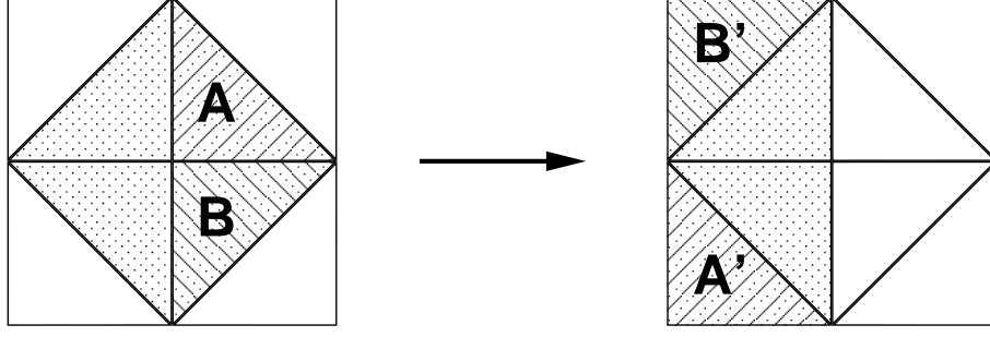
FIGURE 3.12 The two-dimensional analog of the translation of all particles in the right half of the truncated octahedron, our simulation box, to the space between the left half of the truncated octahedron and the containing cube (containing the truncated octahedron), in order to set up the cell list. The rotated square in the middle corresponds to the truncated octahedron and the containing square corresponds to the containing cube. In this analog the translation of the particles corresponds to a translation of all particles in area A to the area A' and all particles in area B to the area B' .
