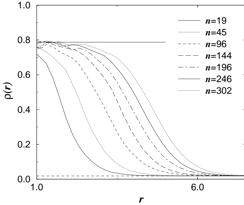
FIGURE 5.3 Density as a function of r , the distance to the center-of-mass of the clusters, for several precritical and critical nuclei at a supersaturation of S = 1.53 ( T = 0.741 , P = 0.01202 ). The thin horizontal dashed line denotes the density in the vapor and the thin horizontal solid line denotes the density in the bulk liquid, which has a chemical potential equal to that of the vapor phase.
